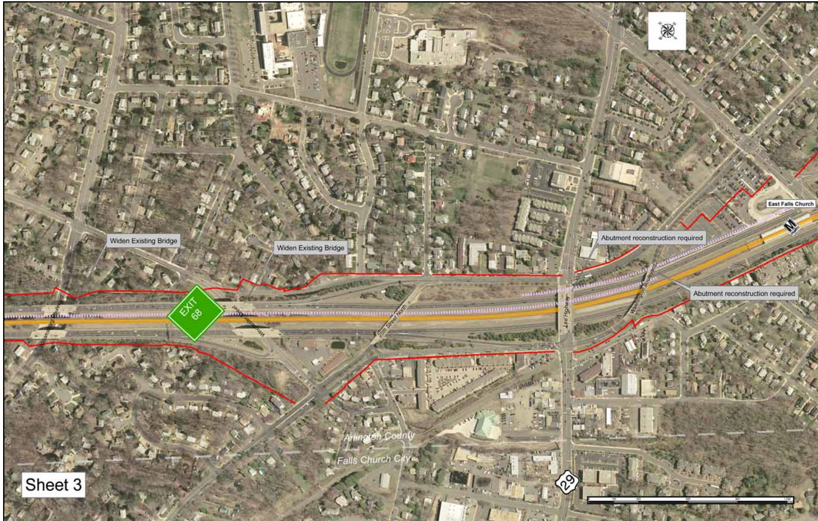
Right-of-way constraints for concepts with additional lane or bus lane.
