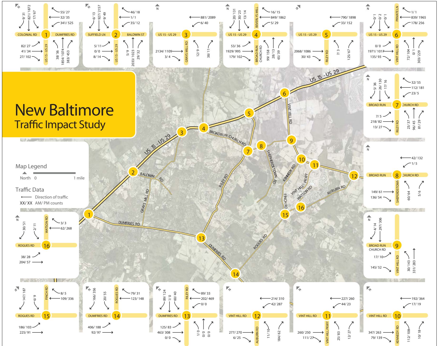
Figure 4: New Baltimore Service District Existing Intersection Volumes (2011)
