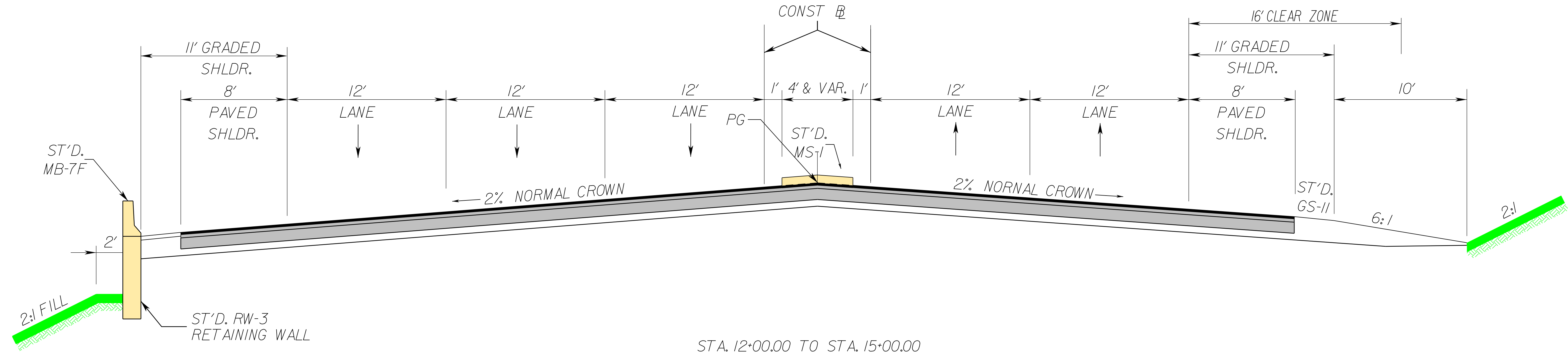
EXIT RAMP 150B / ENTRANCE RAMP TO NB I-81
