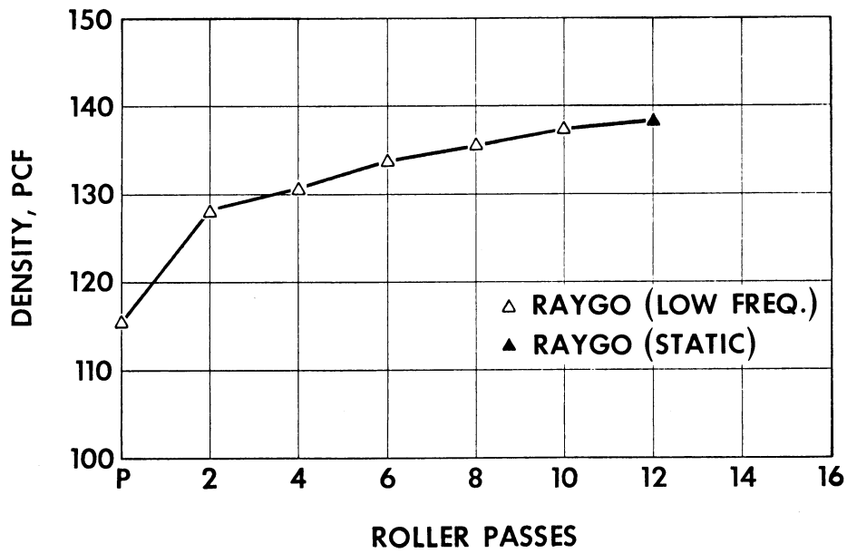
Figure 11. Roller pattern for Raygo roller, low amplitude.
