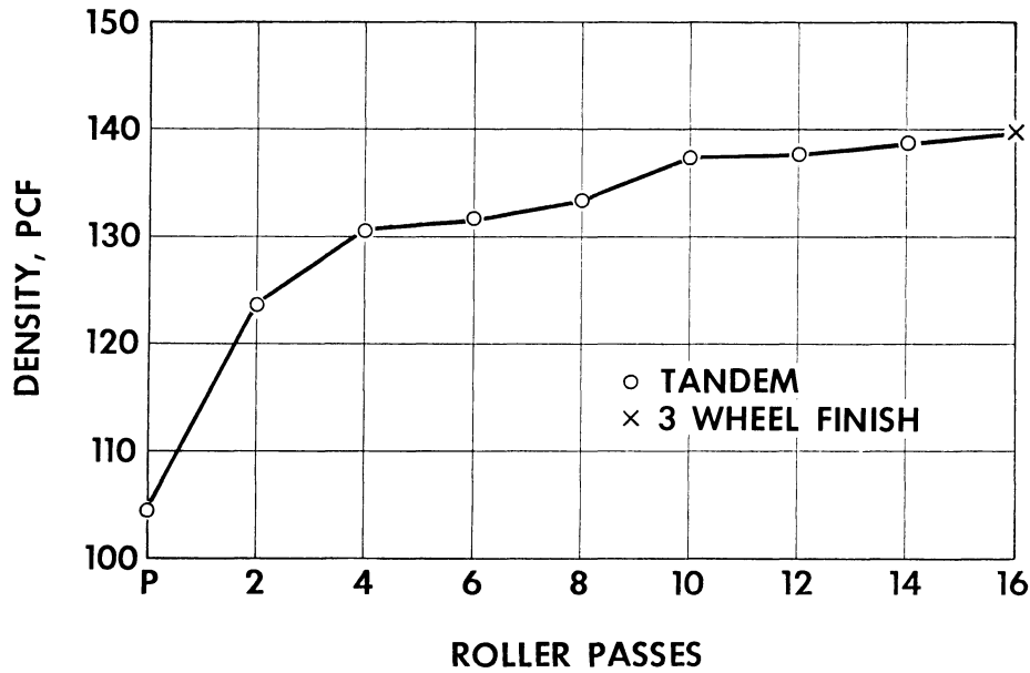
Figure 9. Roller pattern using conventional rollers in reverse sequence.
