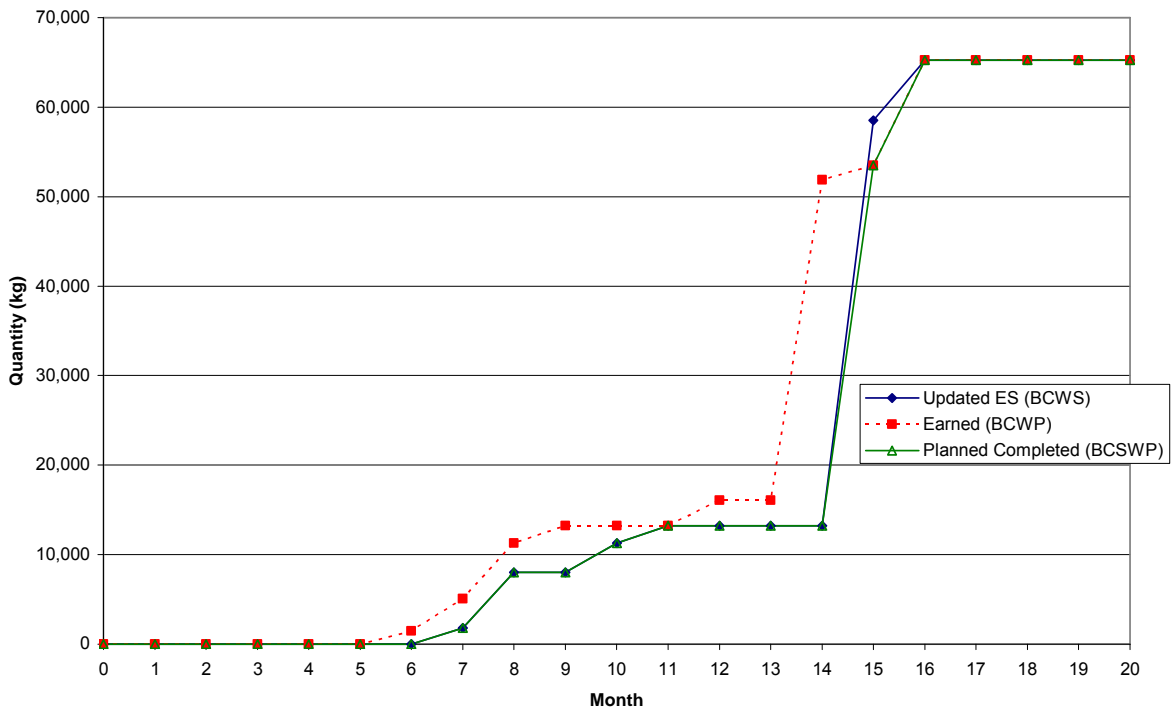
Tom's Creek Interchange Reinforced Steel PPI Curve
