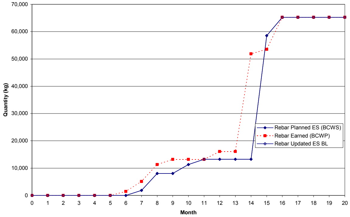
Tom's Creek Interchange Reinforced Steel Commodity Curve
