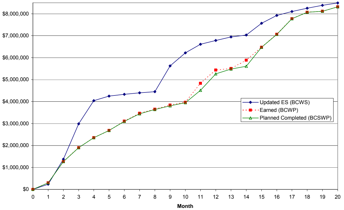
Tom's Creek Interchange Contract Value PPI Curve
