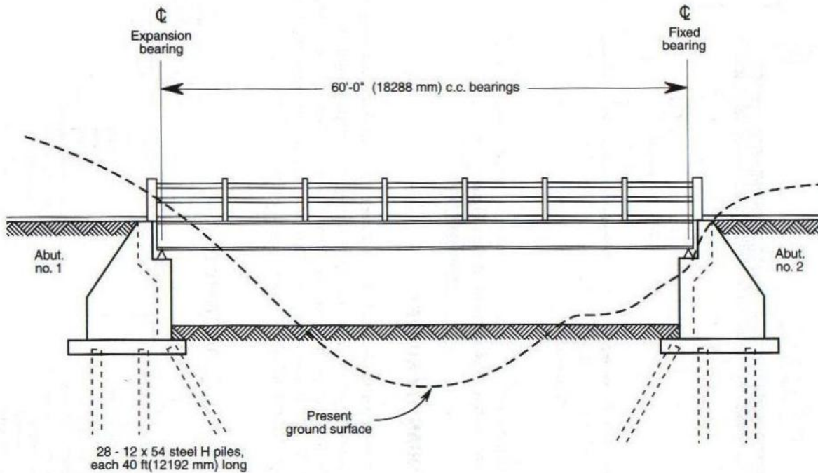
Figure 5: Highway Bridge Profile (Clough et al. 2000)
