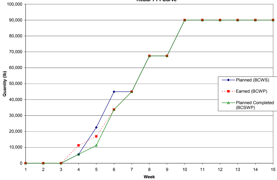
Highway Bridge Project Rebar PPI Curve
