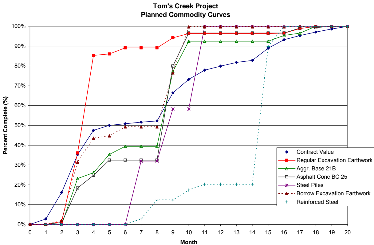
Figure 19: Planned Commodity Curves for Tom's Creek Interchange
