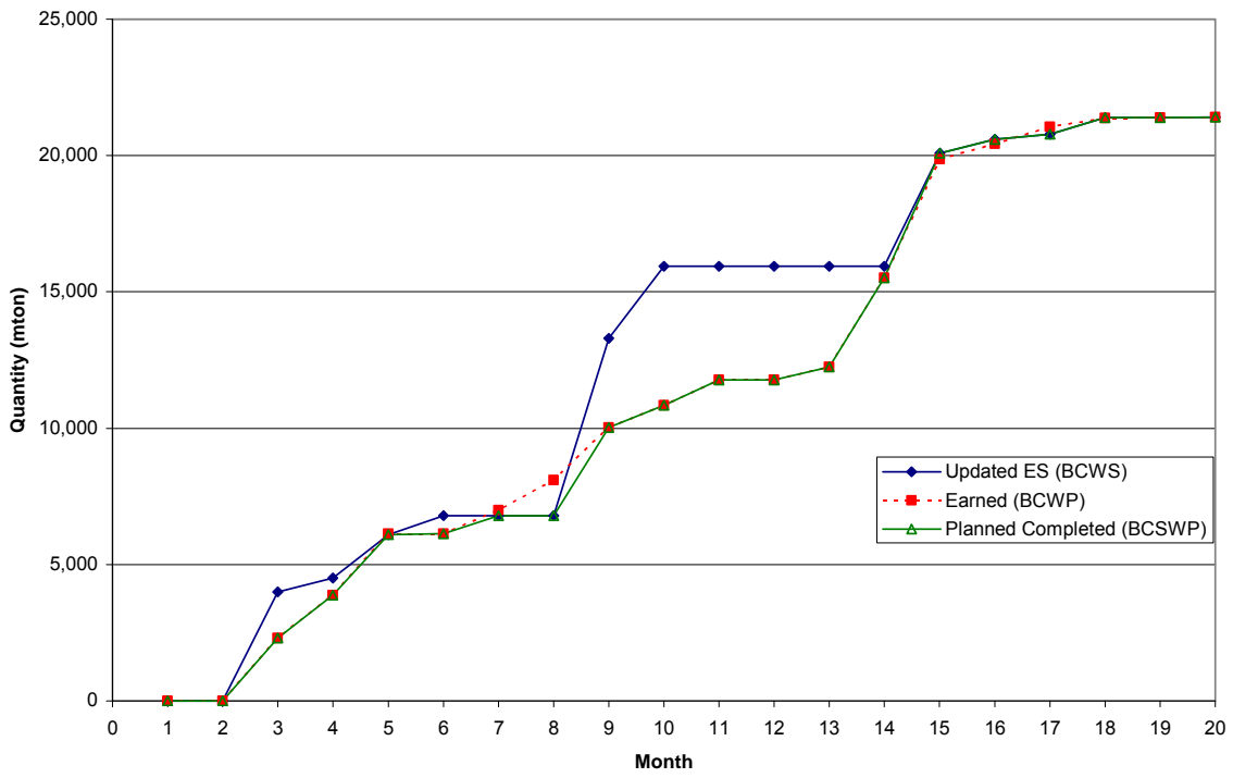
Tom's Creek Interchange Aggr. Base 21B PPI Curve
