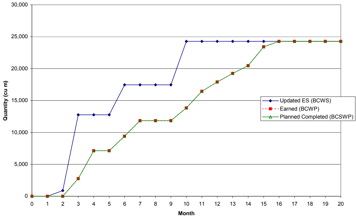
Tom's Creek Interchange Borrow Excavation PPI Curve
