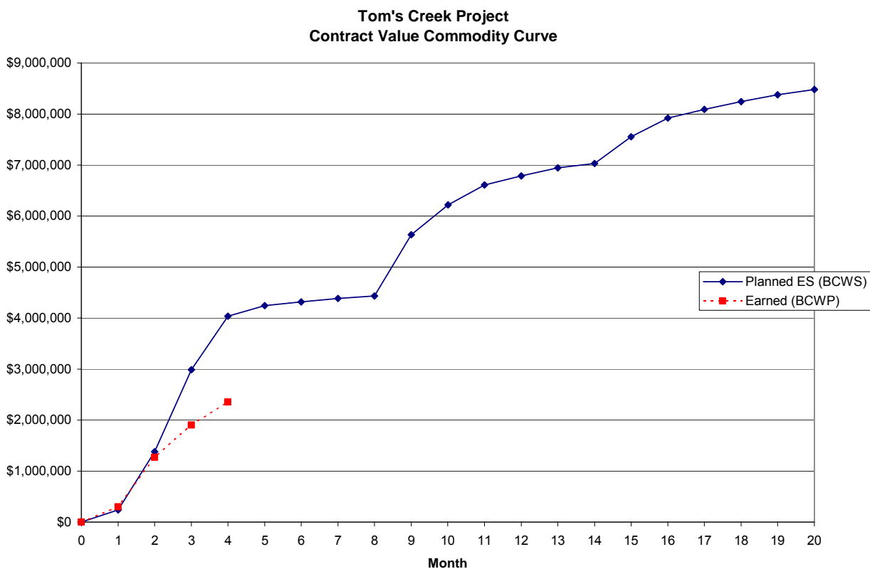
Figure 20: Contract Value of Tom’s Creek Project through Month 4
