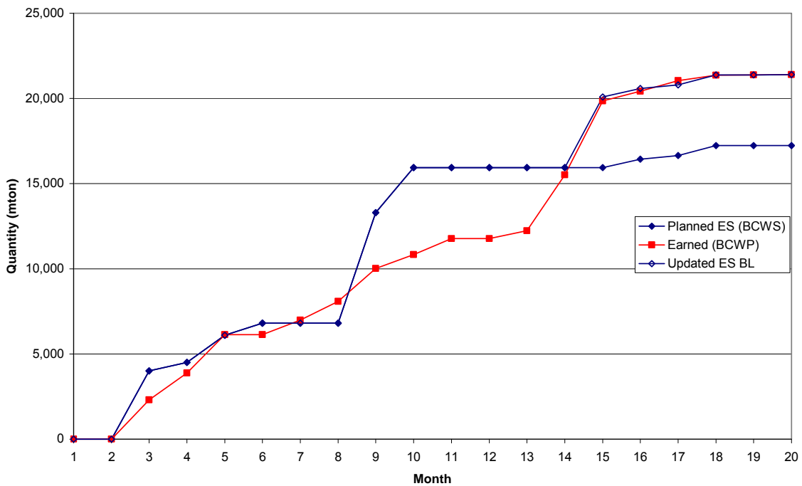
Tom's Creek Interchange Aggregate Base 21B Commodity Curve
