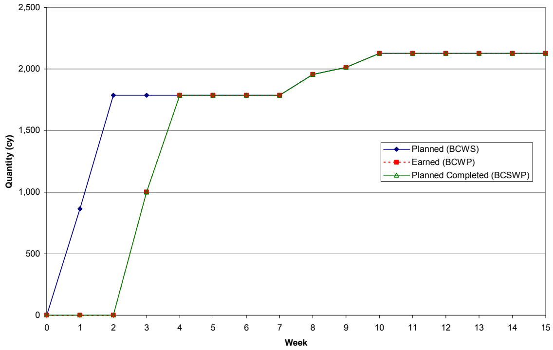
Highway Bridge Project Earthwork PPI Curve
