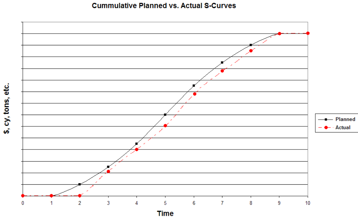
Figure 3: Typical As-Planned versus As-Built S-Curve
