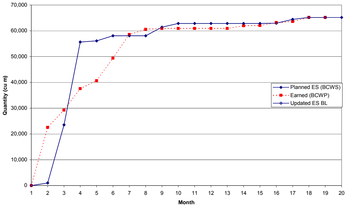
Tom's Creek Interchange Regular Excavation Soil Commodity Curve
