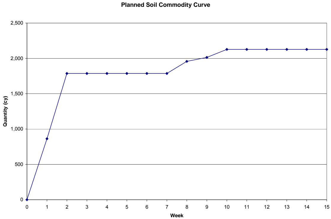
Figure 9: Commodity Curve for Planned Soil Progress
