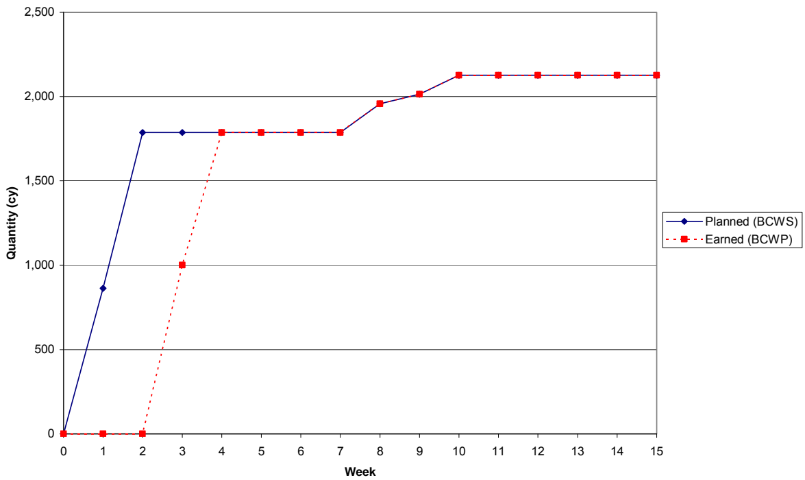
Highway Bridge Project Earthwork Commodity Curve
