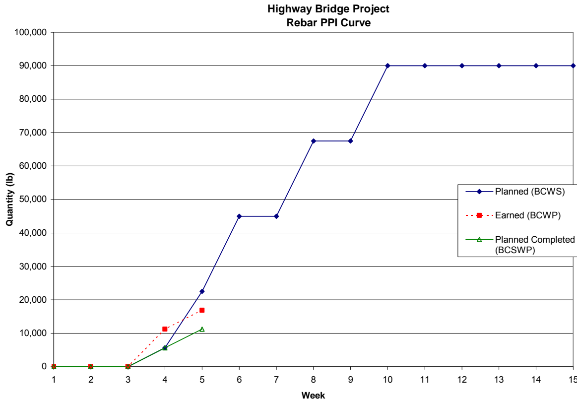
Figure 16: Highway Bridge PPI Commodity Curve for Rebar
