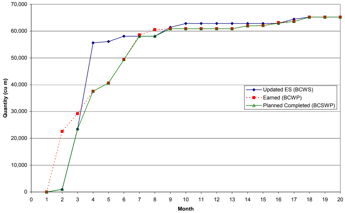
Tom's Creek Interchange Regular Excavation Soil PPI Curve
