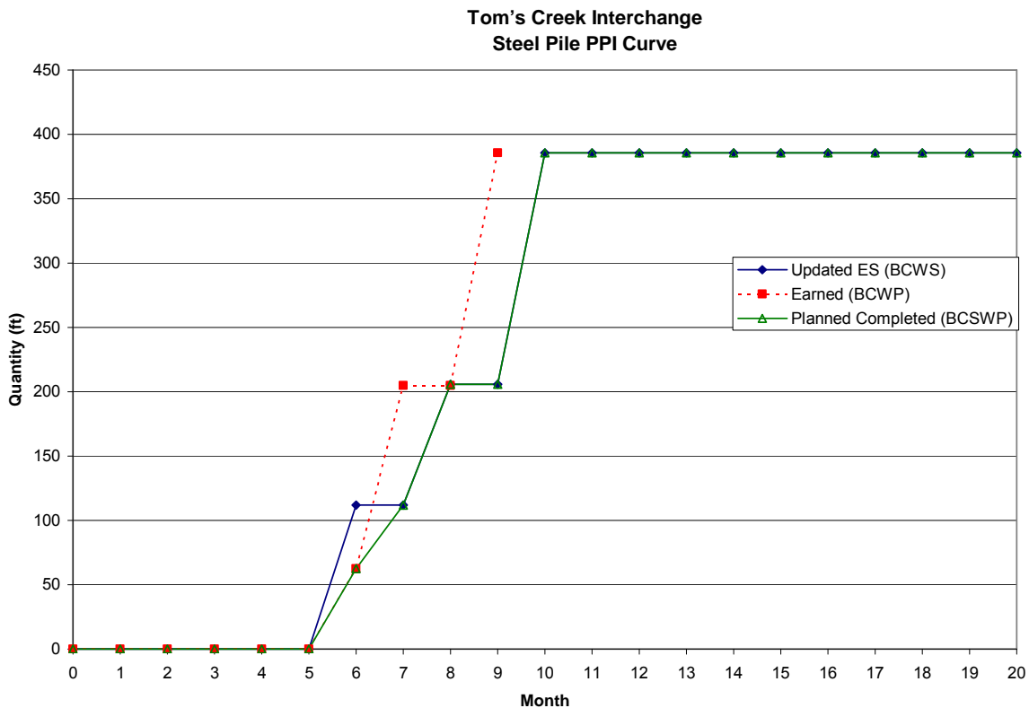
Figure 25: Tom's Creek Steel Piles for PPI through Month 9
