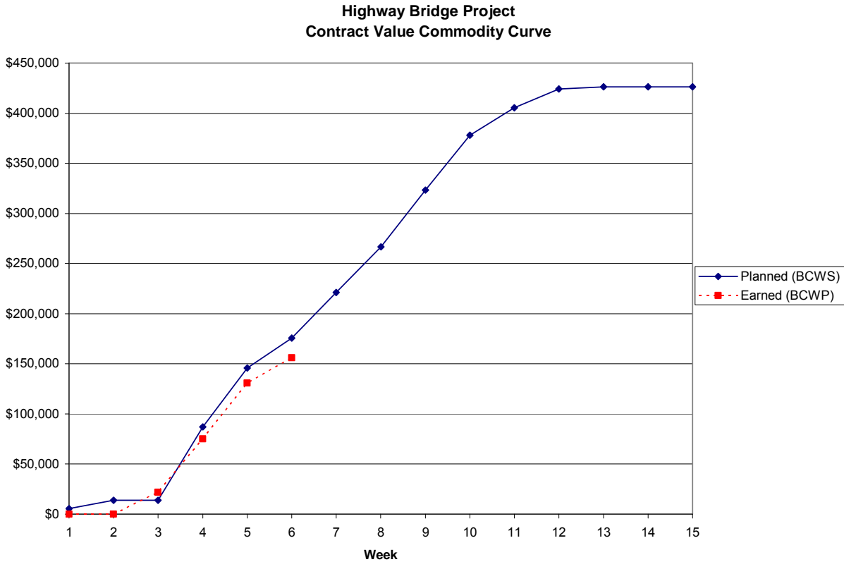
Figure 11: Highway Bridge Contract Value, Week 6
