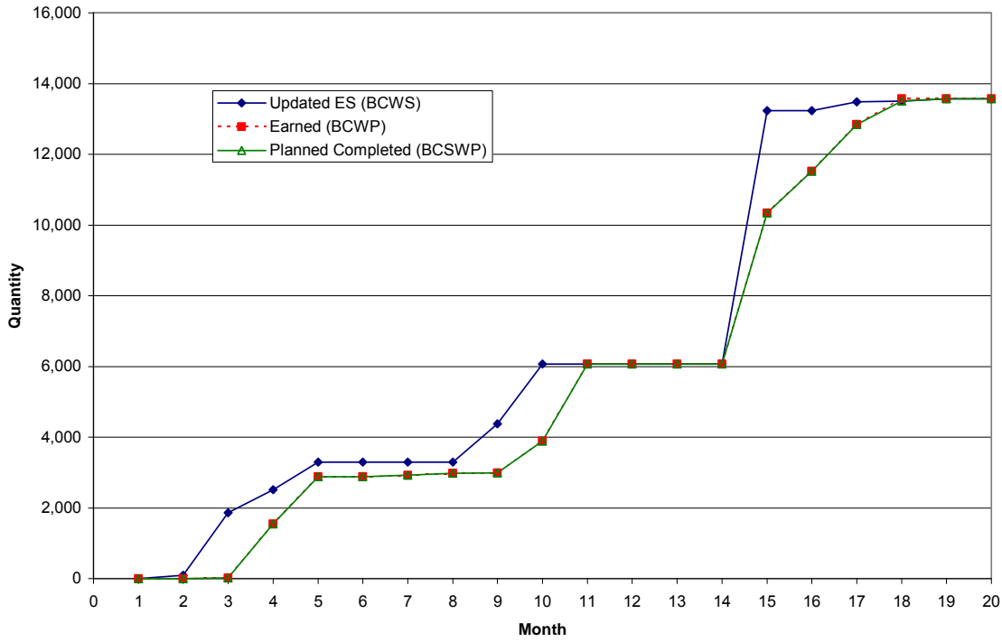
Tom's Creek Interchange Concrete Base Course 25 PPI Curve
