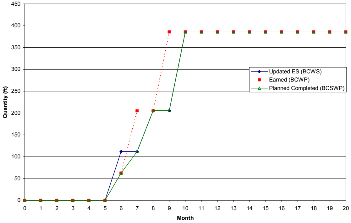
Tom's Creek Interchange Steel Pile PPI Curve
