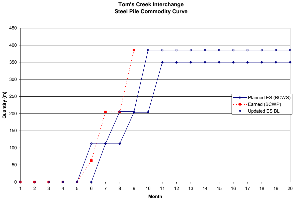
Figure 23: Commodity Curve for Tom's Creek Project's Steel Piles
