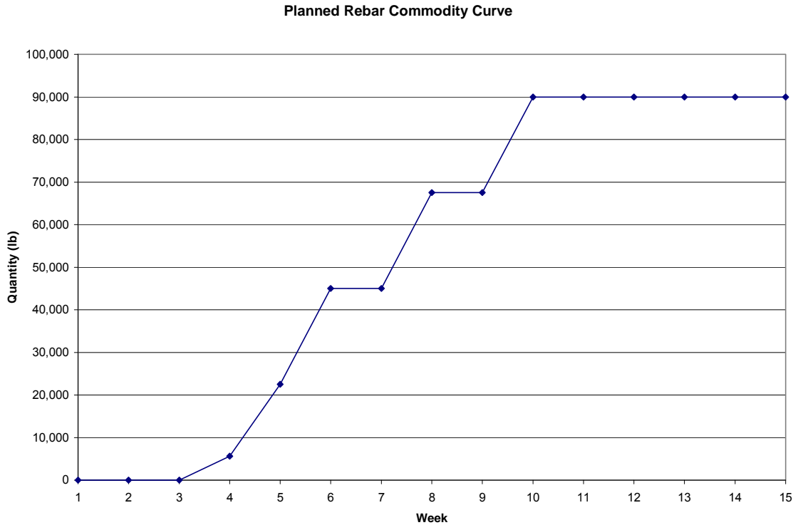
Figure 8: Commodity Curve for Planned Rebar Progress
