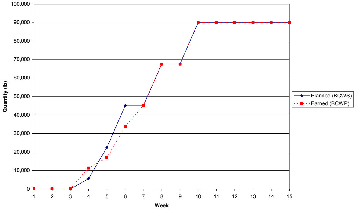
Highway Bridge Project Rebar Commodity Curve
