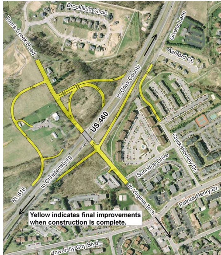
Figure 17: Plan View of the Tom's Creek Interchange
