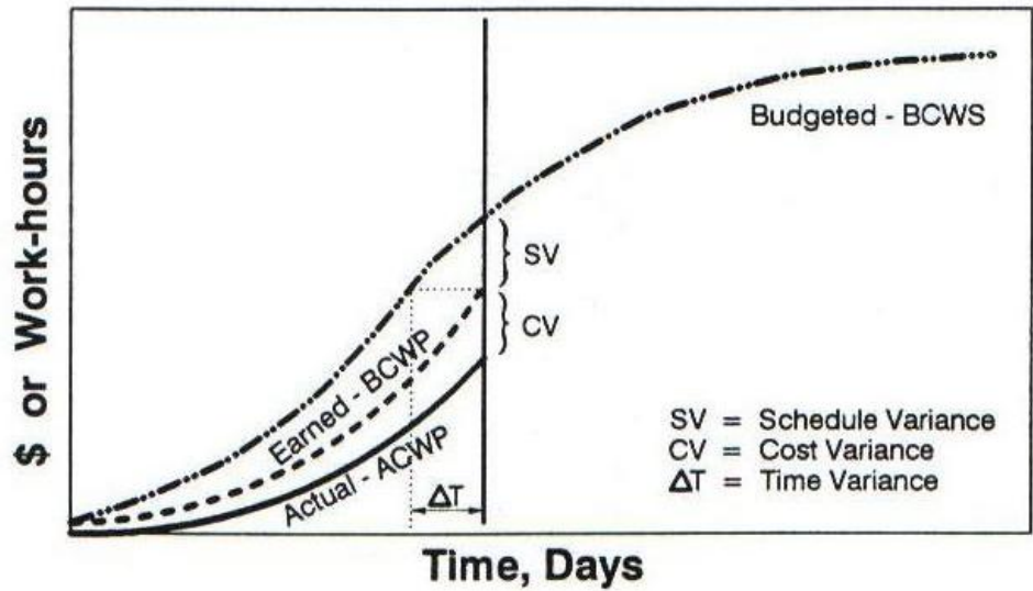
Figure 4: Relationship between Components of the Earned Value Method (Bent 1996)
