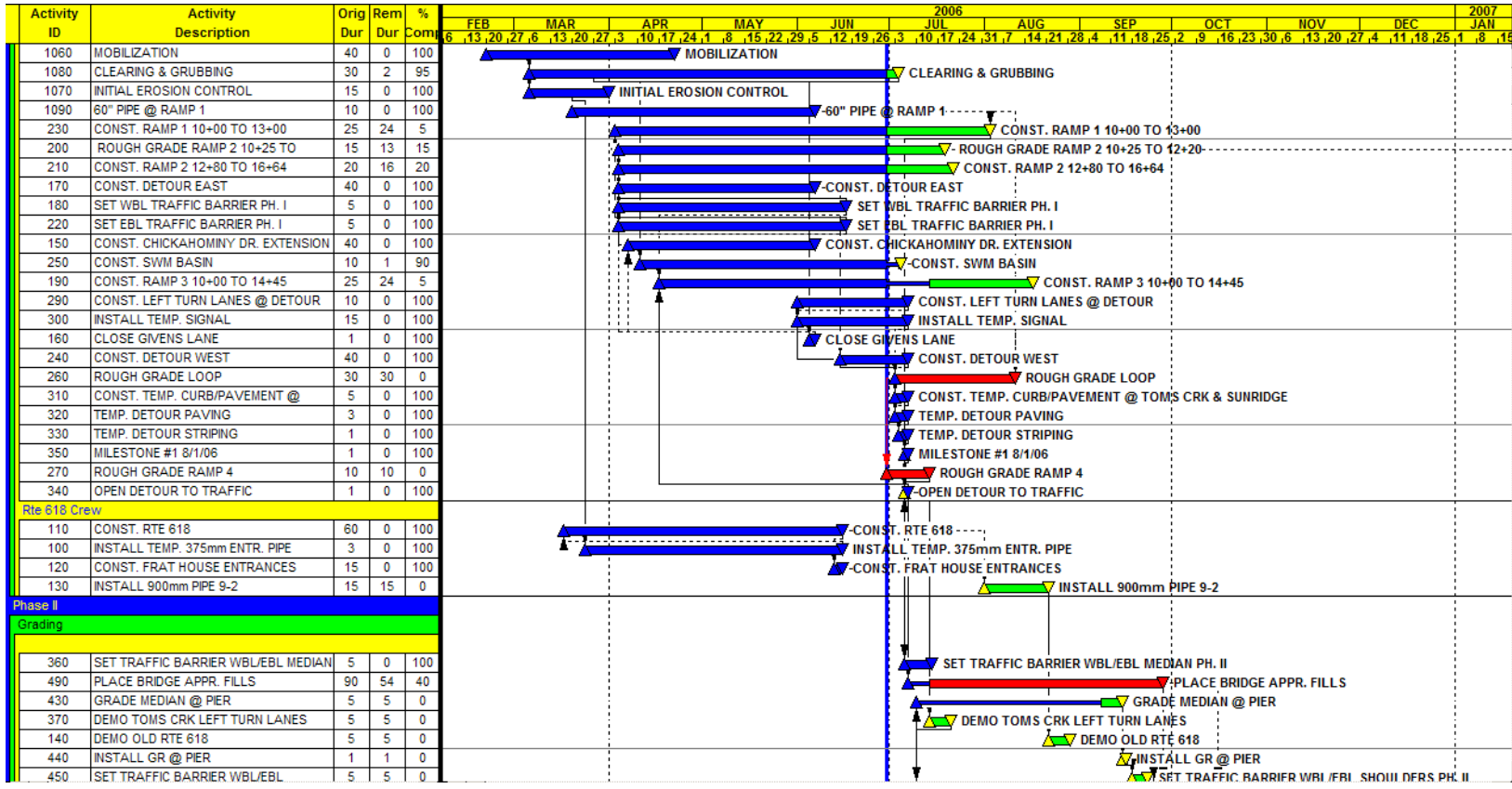
Figure 22: Updated Tom's Creek Schedule Through Month 5
