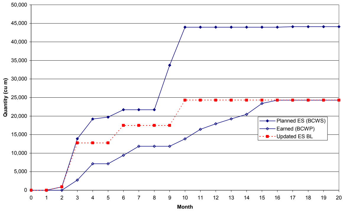
Tom's Creek Interchange Borrow Excavation Commodity Curve
