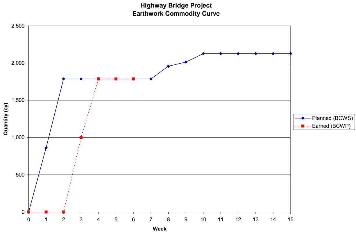
Figure 13: Earthwork Commodity Curve
