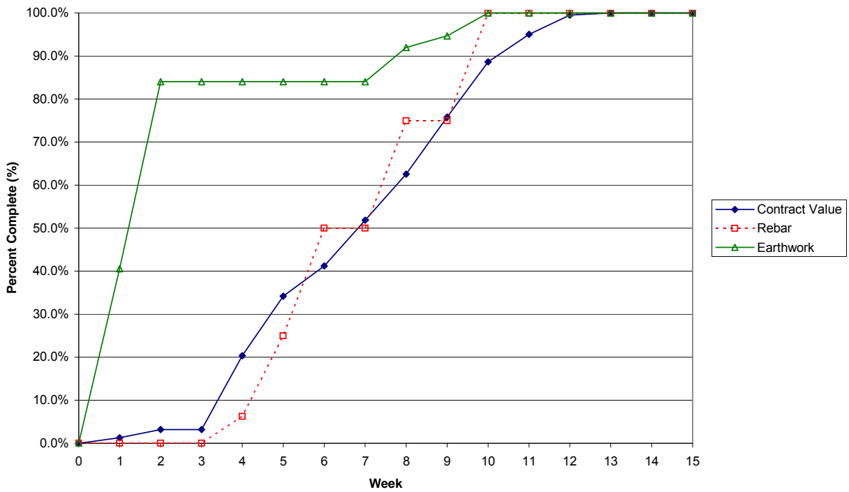
Figure 10: Comparison of the Commodity Curves Planned Progression
