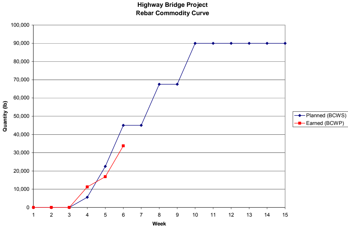
Figure 12: Commodity Curve for Rebar in Week 6
