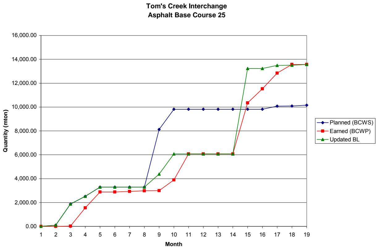
Figure 21: Original and Updated BC 25 for Tom's Creek Interchange Project
